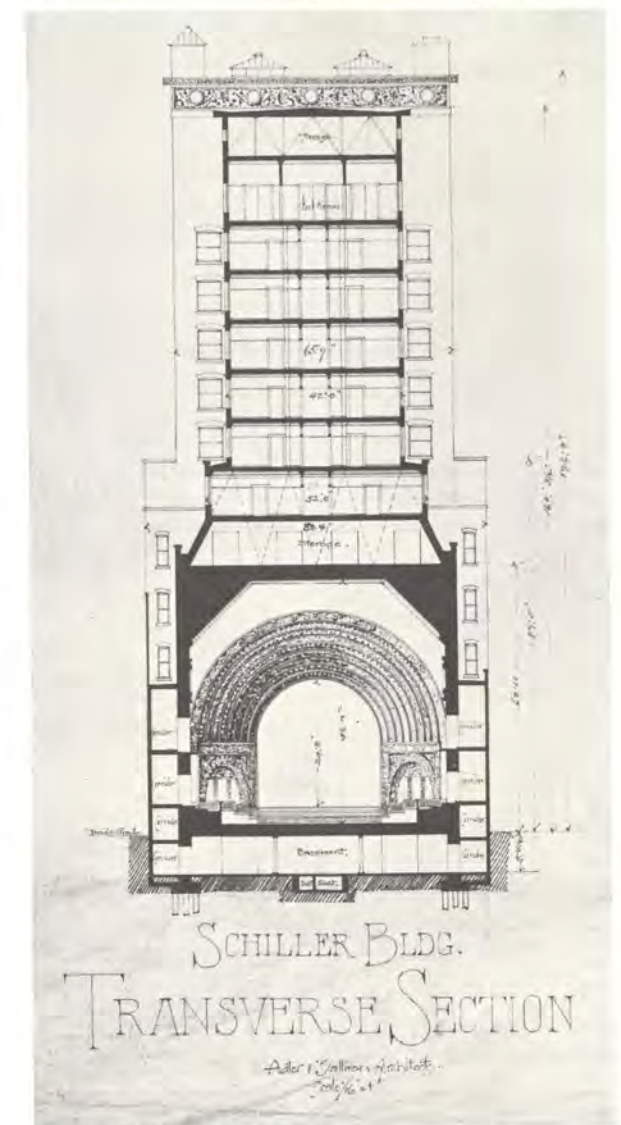
This is a reproduction of Adler and Sullivan's transverse section drawing through the Schiller. The great trusses over the theater are indicated in dotted lines. See longitudinal section on page 23.
