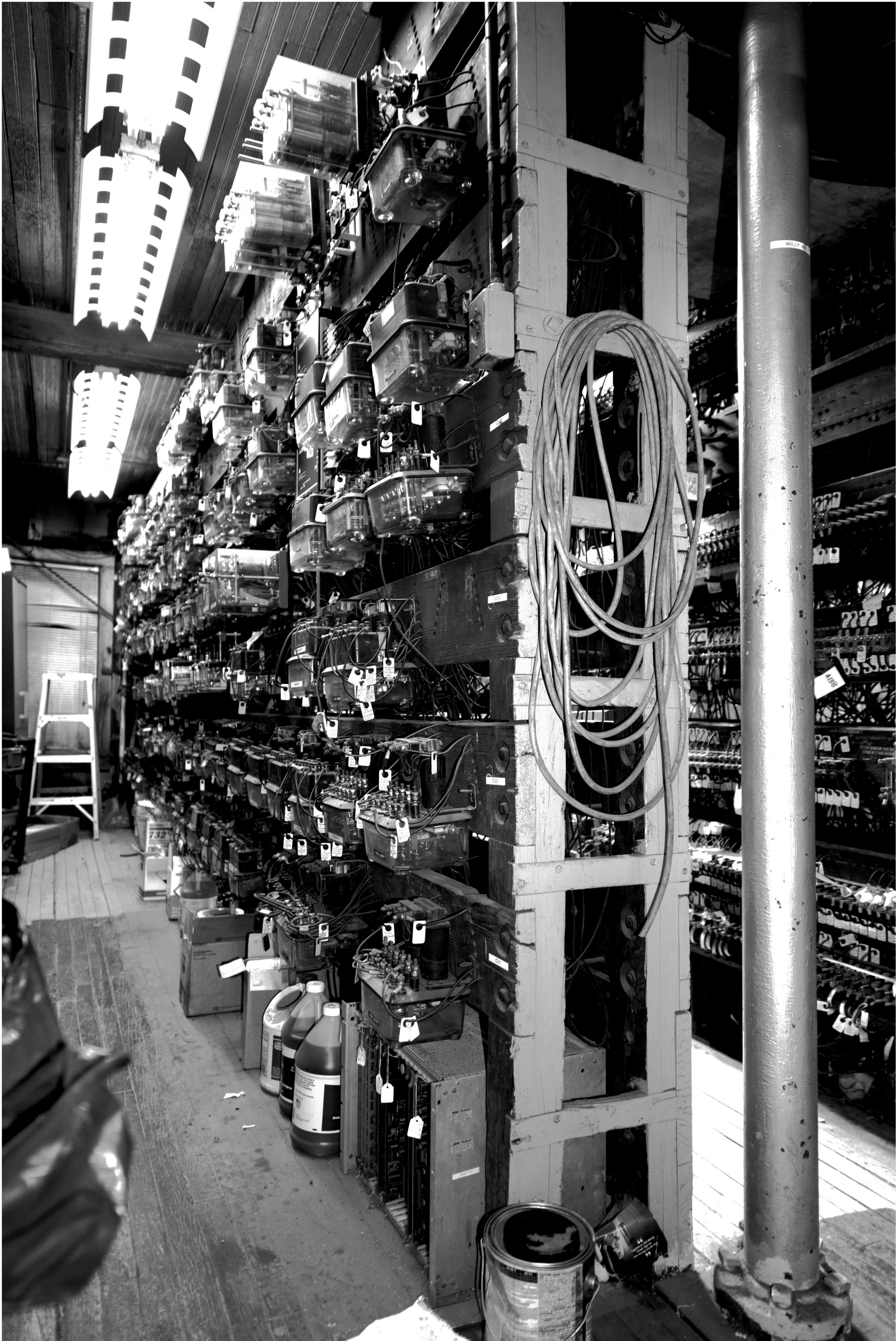
2 of 20 (IL_Cook_16thStreetTower_0002) View of western DC relay rack, first floor, looking northeast.
