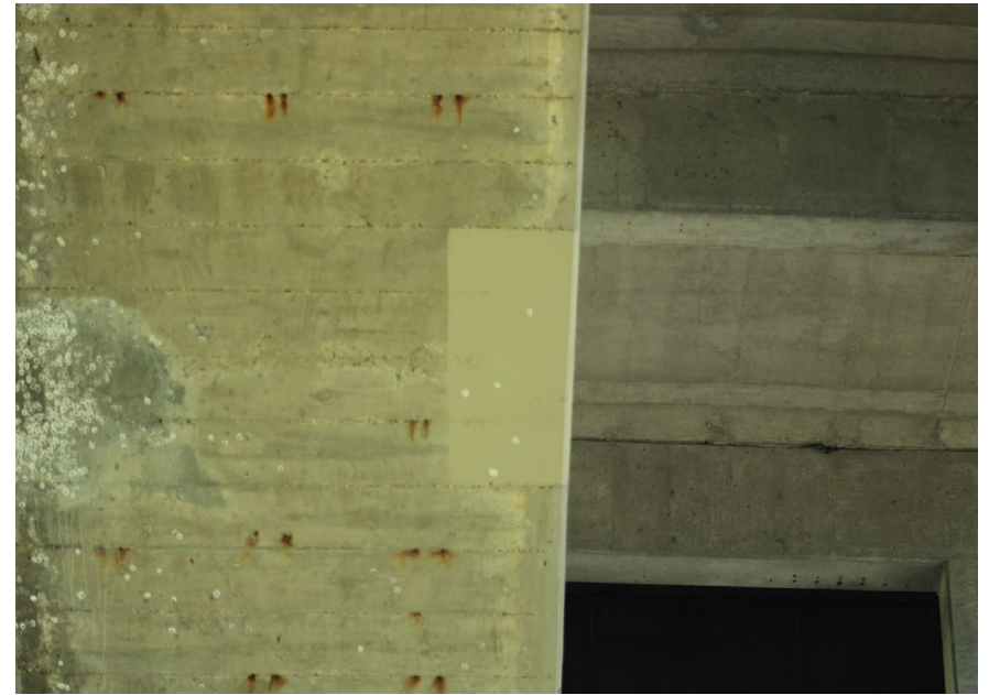
178. Looking North at Patching underneath S.N. 050-0096 Span #6
