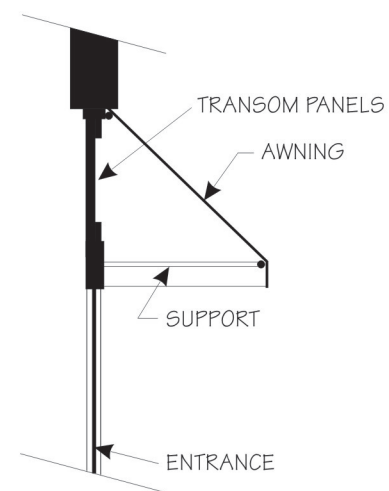
AWNING SECTION
