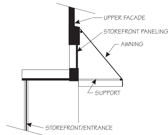
STOREFRONT AWNING SECTION:
