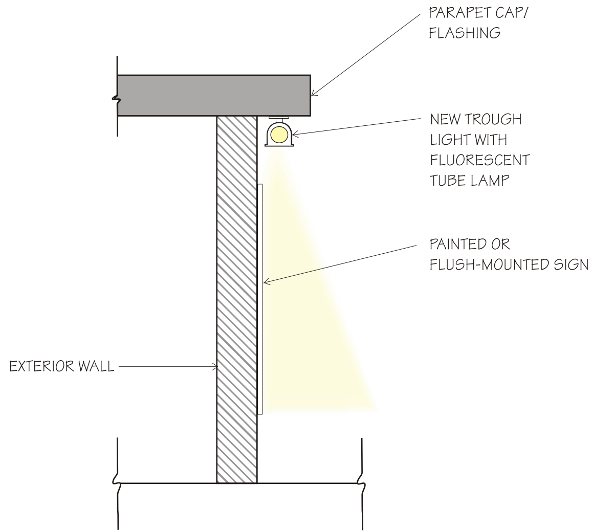
LIGHTING DETAIL - Simplified section through upper exterior wall
