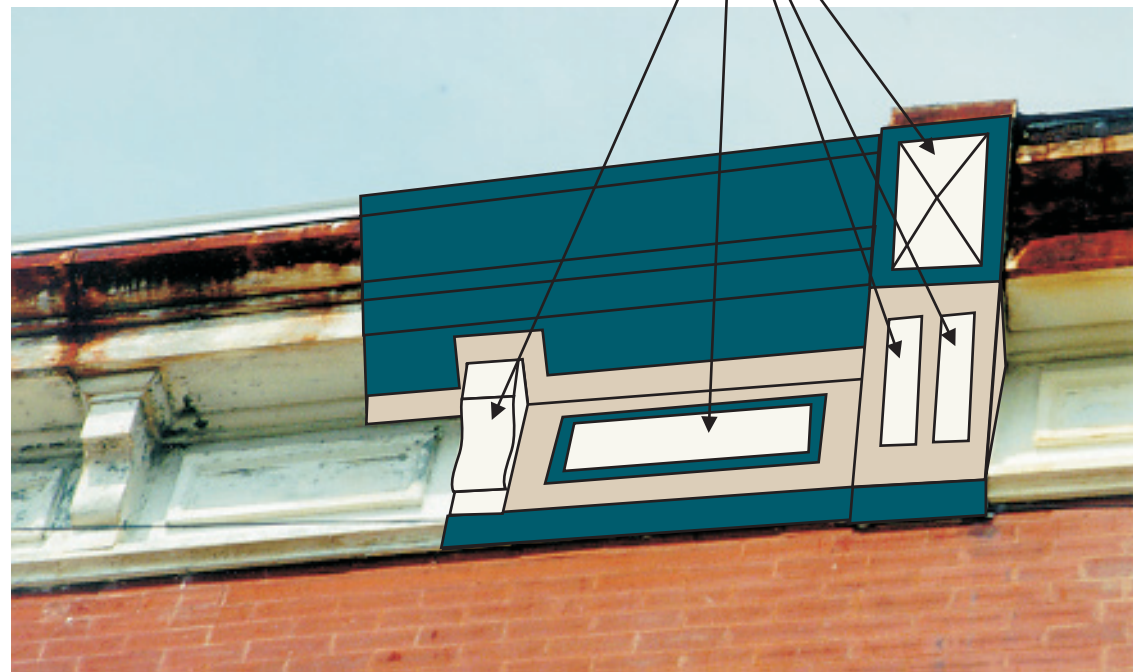
CORNICE DETAIL
