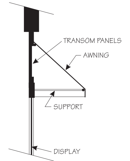
AWNING SECTION:
