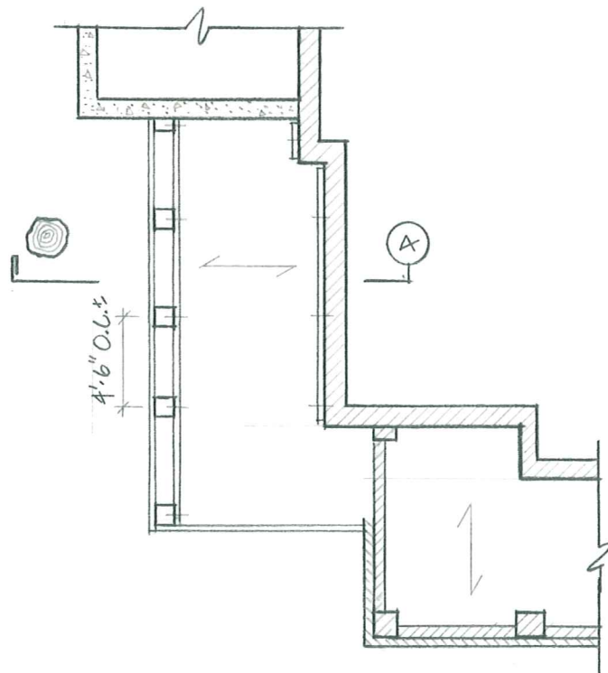
STRUCTURAL PLAN
