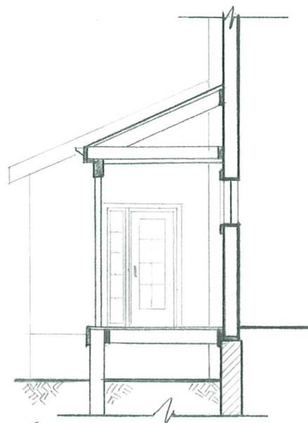
SECTION A
