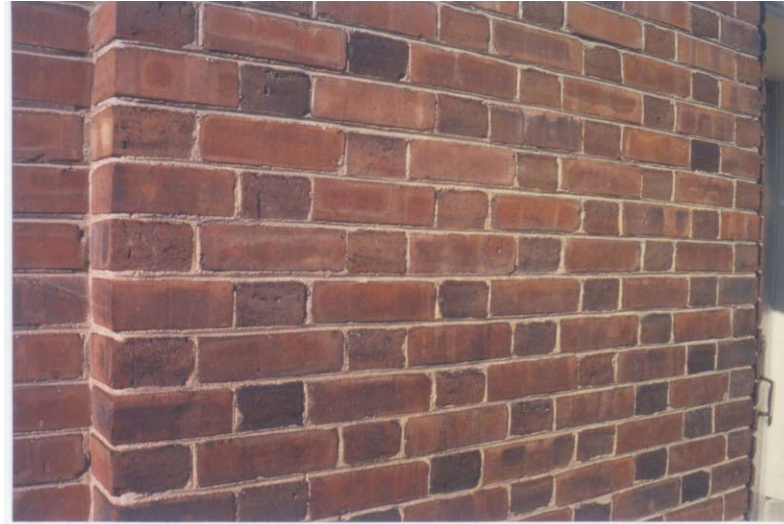
EXAMPLE OF FLEMISH BOND
