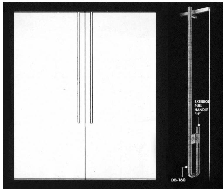
Blumcraft Series 1301 doors in combination with a floating transom bar. Dead bolt lock housing DB-160 with exterior pull handle "H". Exposed metal to match the champagne finish of the storefront.
