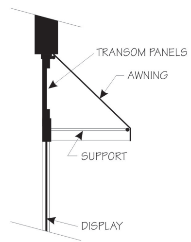
AWNING SECTION
