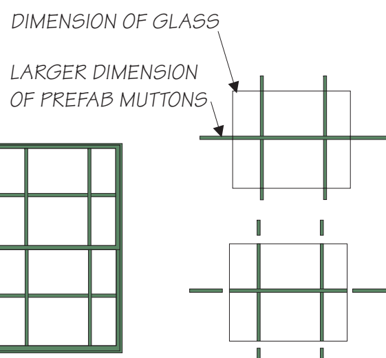
SUGGESTED CONFIGURATION THAT MAINTAINS EXISTING MUTTON PATTERN
