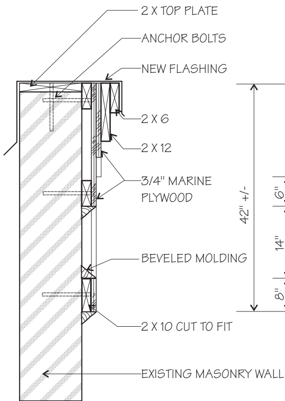
SECTION
