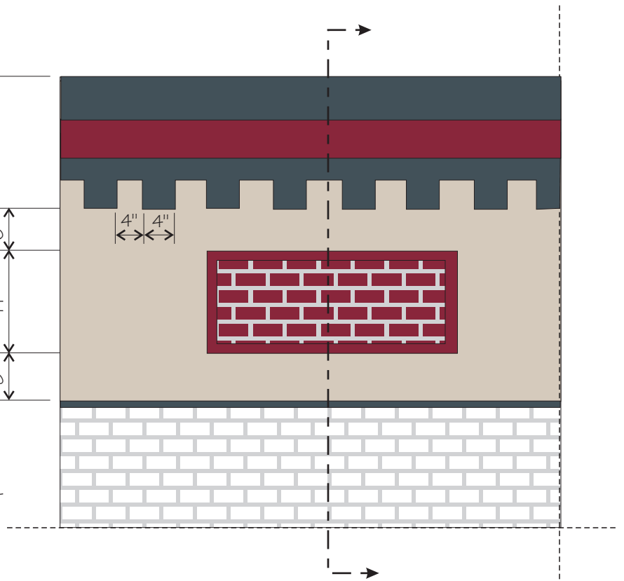
ELEVATION DETAIL
