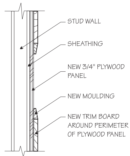
TYPICAL PANELING DETAIL
