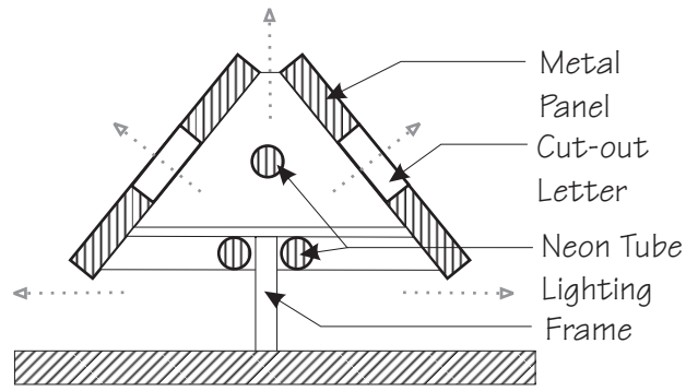
SECTION CUT THROUGH SIGN
