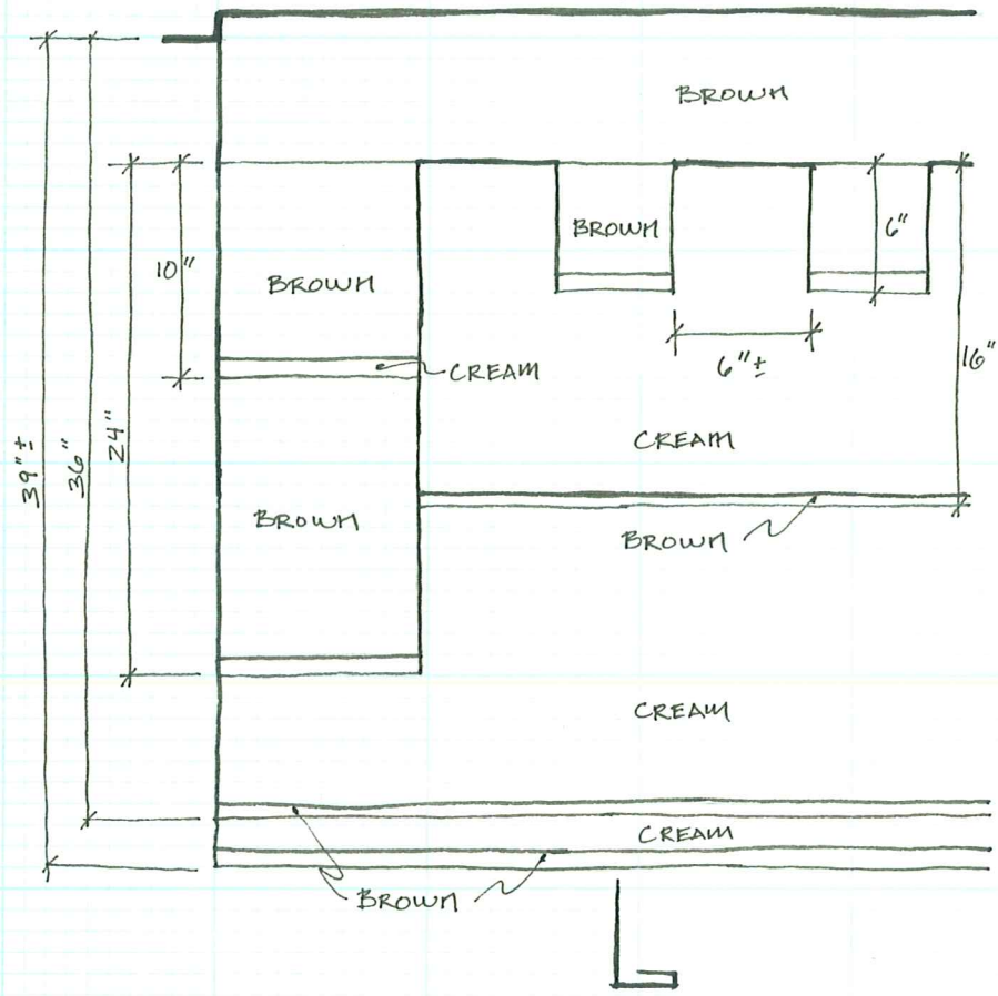
ELEV. DETAIL
