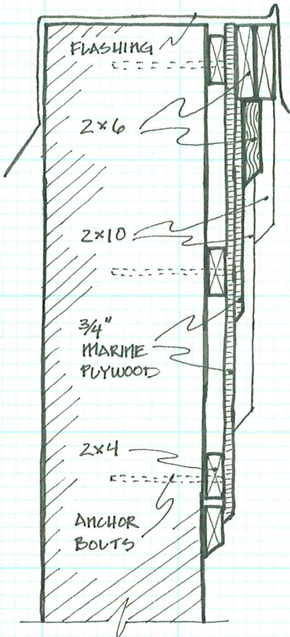
SECTION "A"
